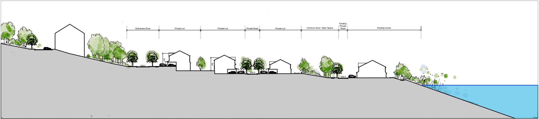
Section C-C
